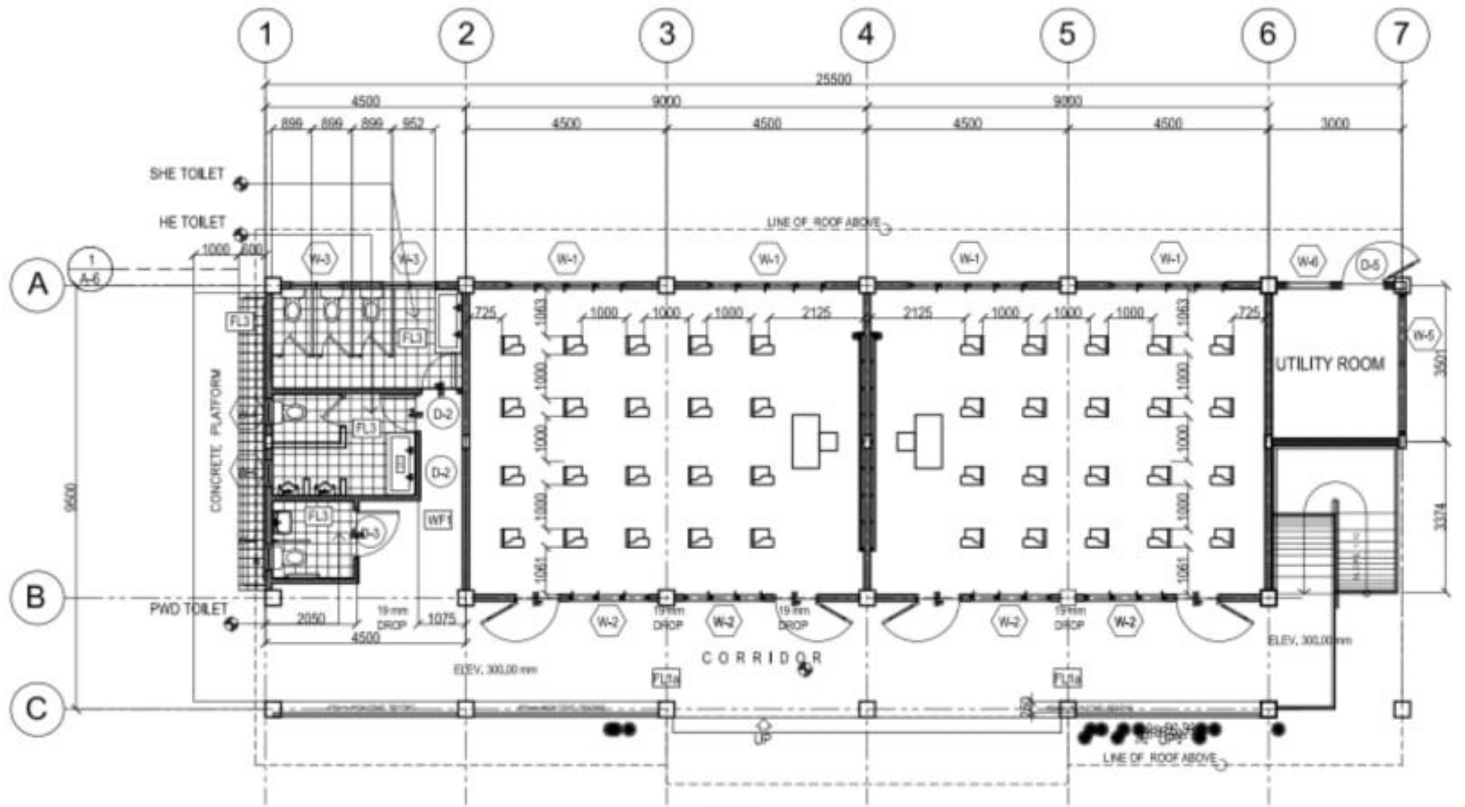
2 FLOOR PLAN A-2 1:100M SCALE
