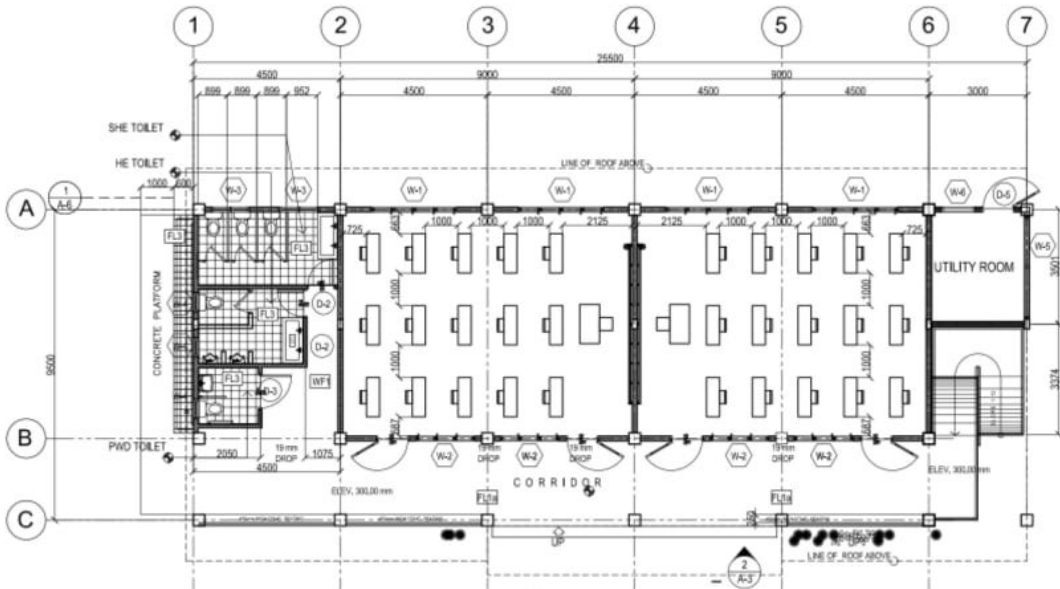
2 FLOOR PLAN A-2 1:100M SCALE
